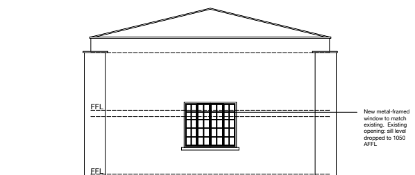
NORTH ELEVATION
