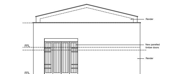
SOUTH ELEVATION
